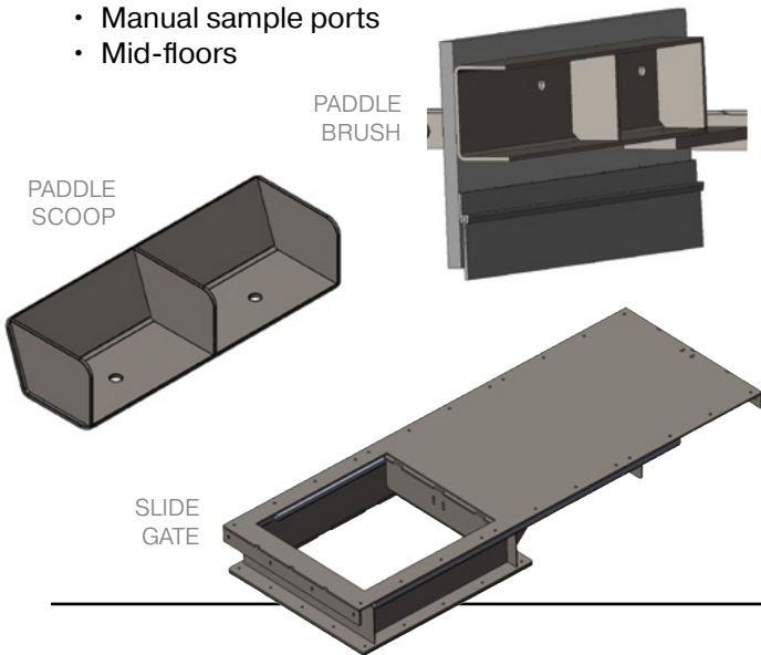
MANUAL SAMPLE PORT
